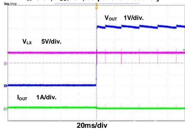
Figure 19. output short recovery.
