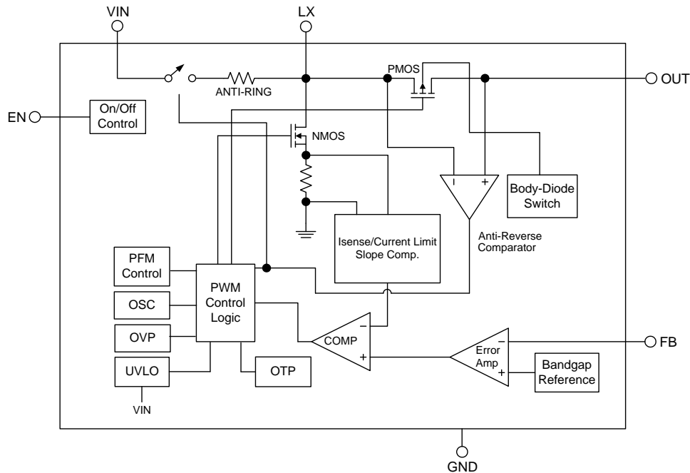
Figure 3. Block Diagram of FP6715
