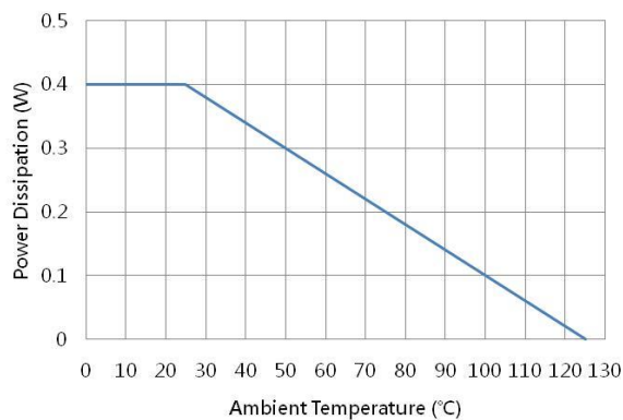
Figure 20. SOT-23-6 Package P_D Derating Curve
