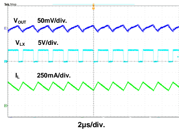
Figure 15. Switching Waveform
