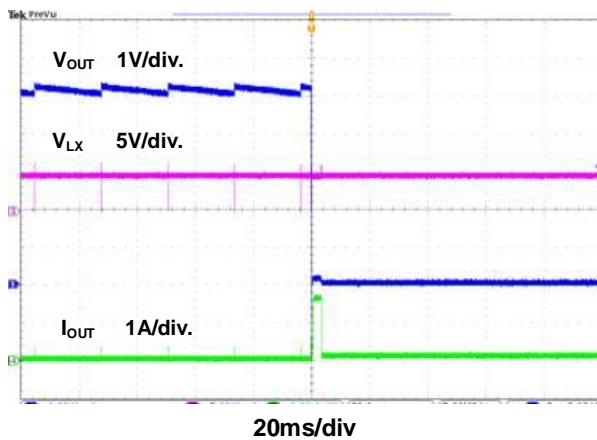
Figure 18. output short to GND.
