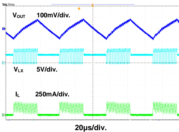
Figure 14. Switching Waveform
