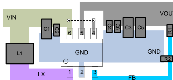
Figure 21. Layout Diagram
