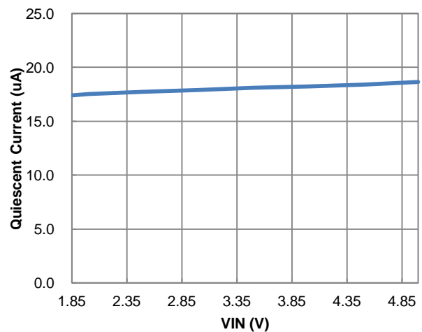
Figure 7. Quiescent Current vs. VIN
